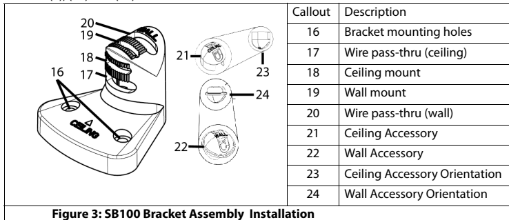
Figure 3: SB100 Bracket Assembly Installation
